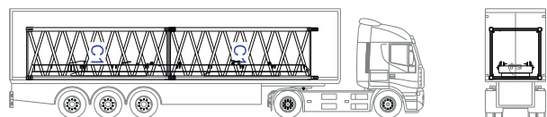
2xC1-CL4-2xCP3
