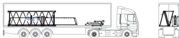
L42a-L42b-C1-P3
