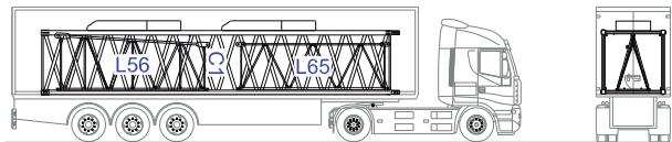
C1-L56-L65-2xCP2
